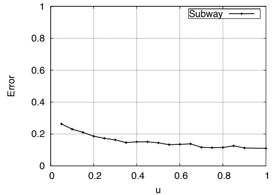
Fig. 7. The error versus SpotME's penetration rate u among subway passengers.
