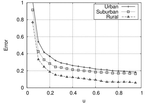
Fig. 6. The error versus SpotME's penetration rate u among vehicular drivers.
